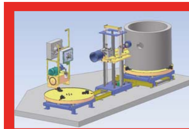
Basic Machine with One Traversing Turntable One 48" Turntable and Two Spindles
